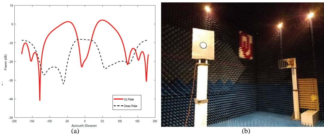
Figure 6: Example of improved antenna modeling, (a) Measured DME antenna pattern, (b) EM chamber setup.
