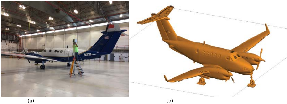
Figure 2: (a) 3D laser scanning of King Air, (b) Resulting mesh model in simulation environment.
