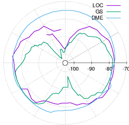
Figure 12: Yaw signal sensitivity measurements (dBm).
