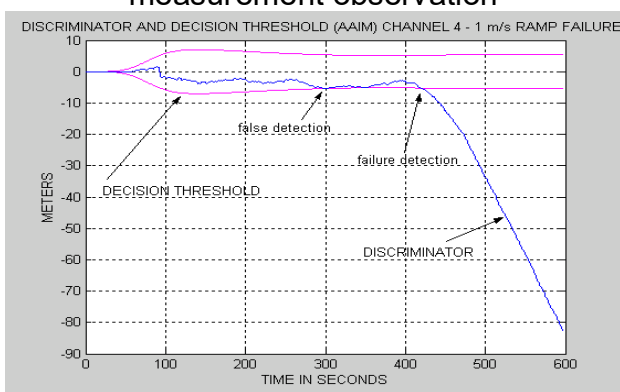
Figure 13. Discriminator deviation due to correlated noise
