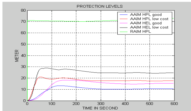
Figure 9. Horizontal protection levels.
