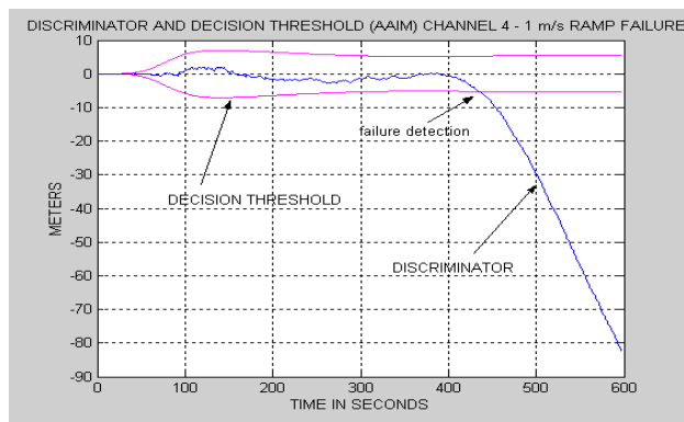
Figure 10. Discriminator deviation due to satellite failure causing ramp
