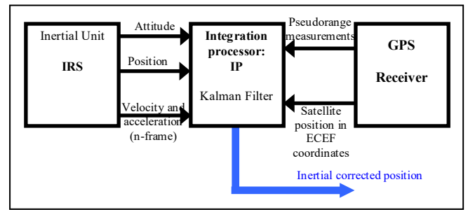
Figure 3. GPS/IRS architecture
